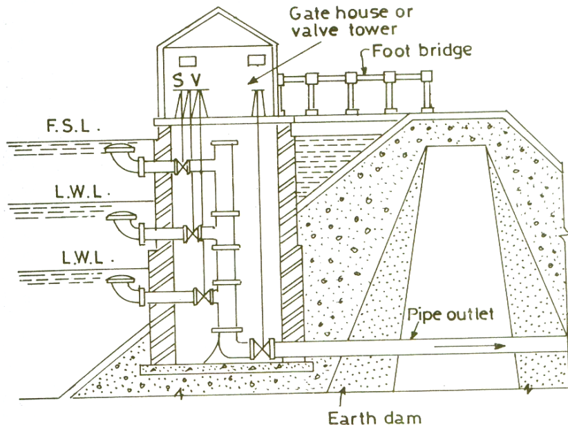
Fig. 4.3 (Reservoir Intake)
