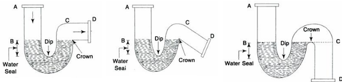
(a) P-Trap
