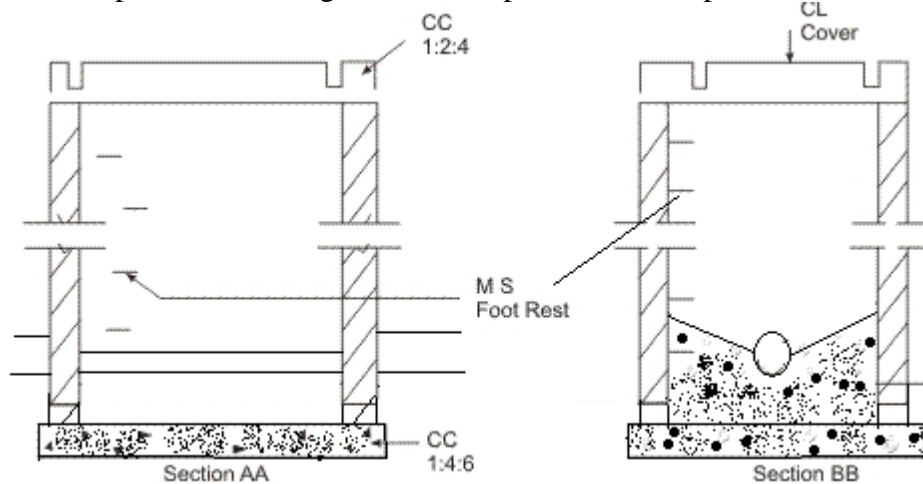
Shallow Manhole
