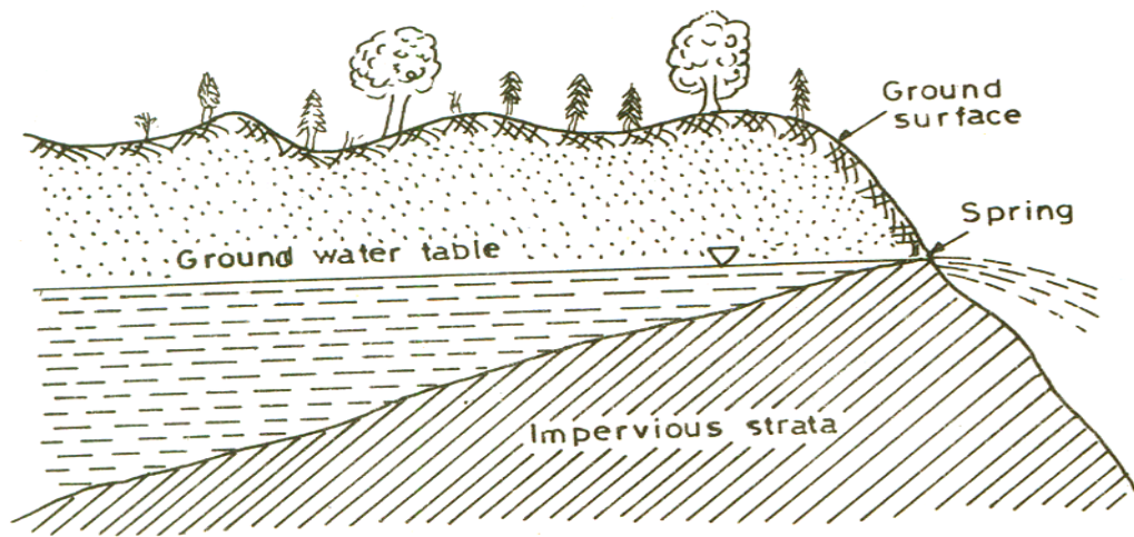
Fig. 3.1(Shallow Spring)
