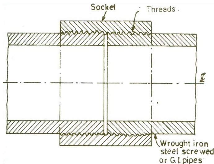
Fig. 4.10 (Screwed & Socket Joints)
