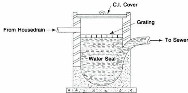
Gully Trap
