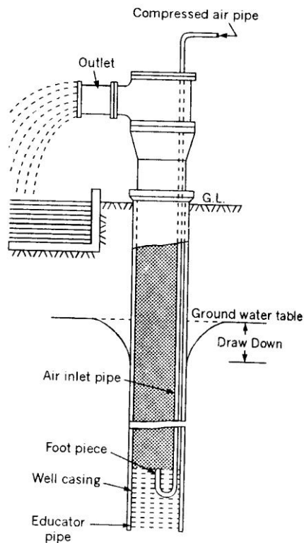
Air lift pump
