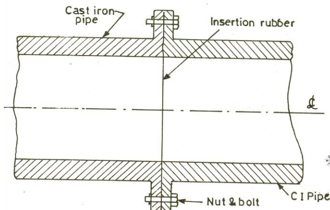
Fig. 4.6 (Flanged Joint)
