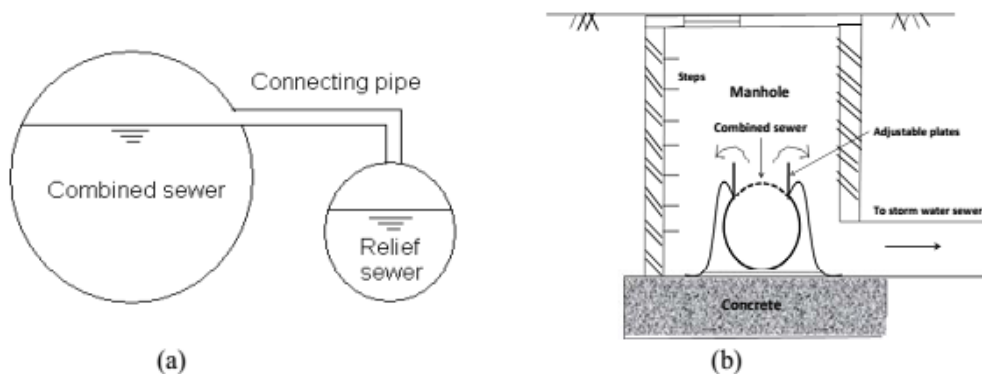
(a)Side flow weir (b) Overflow weir arrangement
